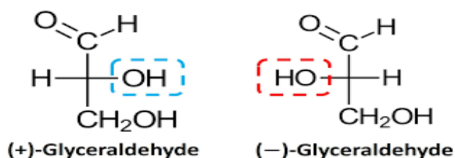
Figure 3: D and L Glyceraldehyde
